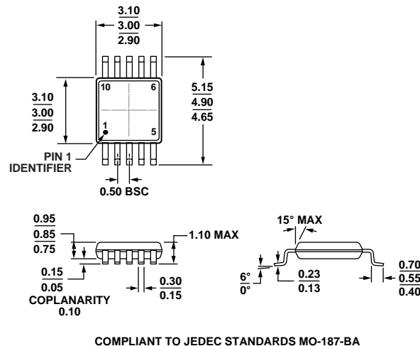
COMPLIANT TO JEDEC STANDARDS MO-187-BA Figure 32. 10-Lead Mini Small Outline Package [MSOP] (RM-10) Dimensions shown in millimeters
