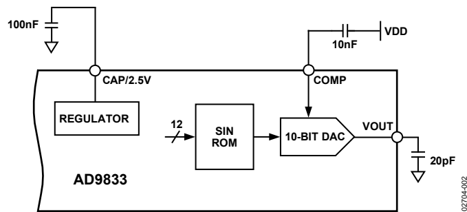
Figure 2. Test Circuit Used to Test Specifications
